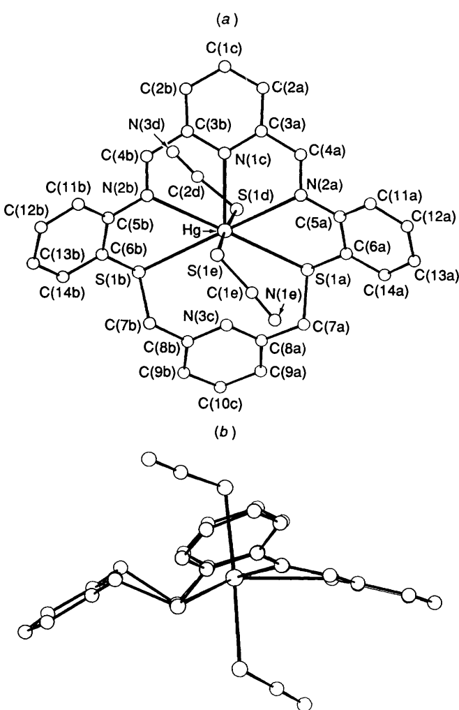
Fig. 3 Structure of [\text{HgL}^1(\text{SCN})_2] \cdot \text{MeOH} : (a) view showing atom labelling and metal-donor interactions; (b) view showing macrocycle conformation and disposition of the mercury atom
